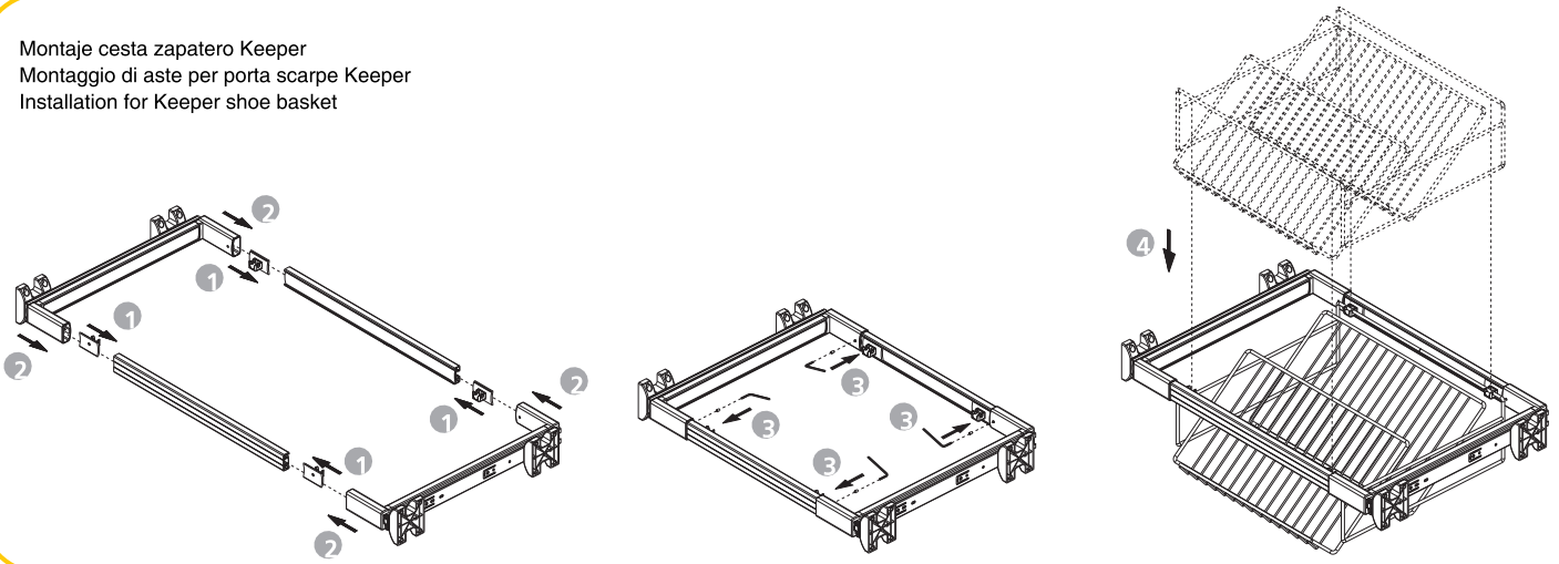
Montaje distanciador Keeper Montaggio distanziali Keeper Installation for Keeper spacer
